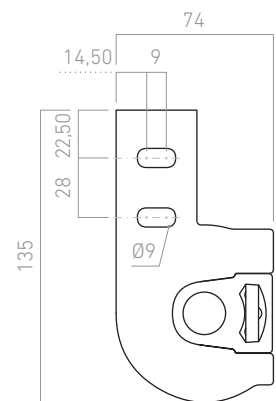
Top bracket
